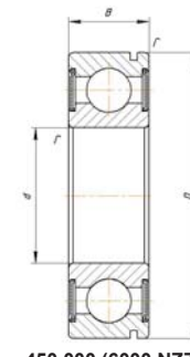
450 000 (6000 NZZ) 750 000 (6000 N2RS)
