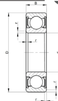
180 000 (6000 2RS)
