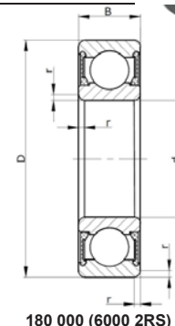
180 000 (6000 2RS)
