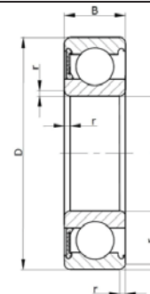
160 000 (6000 RS)
