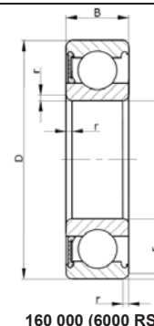
160 000 (6000 RS)
