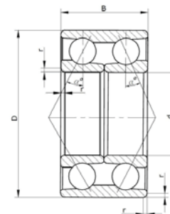
3 086 000 (3000 D)
