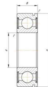
450 000 (6000 2ZZ) 750 000 (6000 2RSN)
