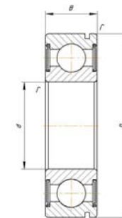
450 000 (6000 NZZ) 750 000 (6000 N2RS)
